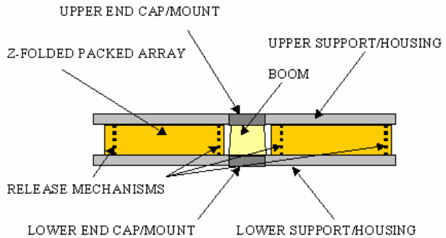
Figure 6: Stowed Configuration
